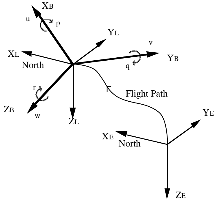
Figure 3 Inertial (E), Local (L), And Body (B) Axes
